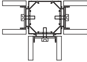
3 Way Connector
