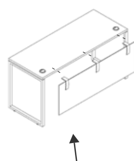
2 Screw modesty panel into table top from underneath the table using the connectors
